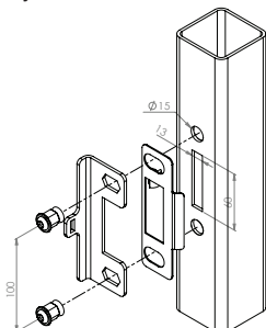
MLK Mortice Lock Keep
