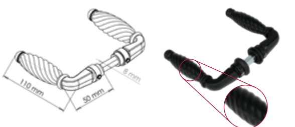
T Twisted handle set
