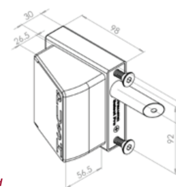
Right hand lock shown
